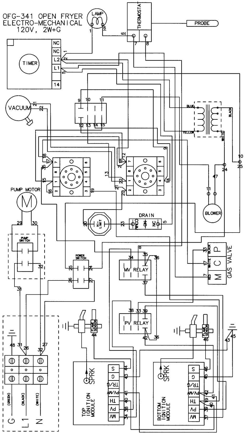
Drain switch wired N/C
