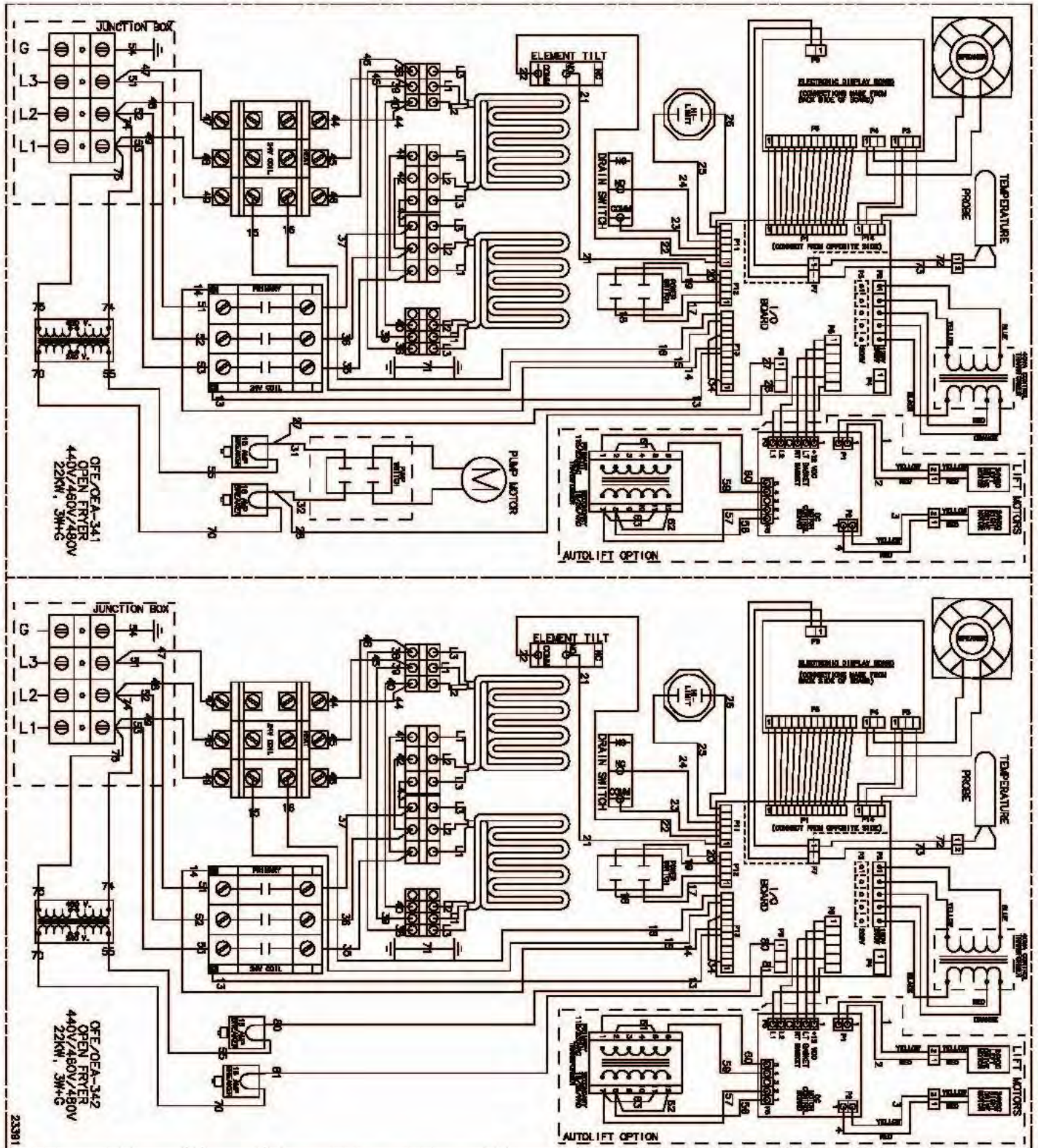
Drain switch wired N/C
