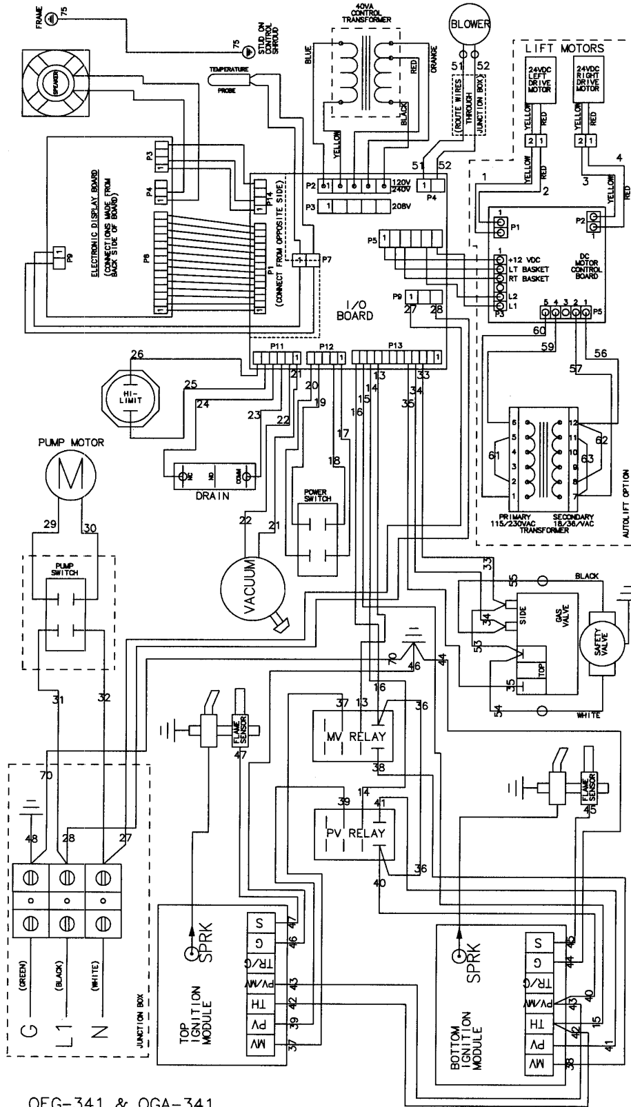
OFG-341 & OGA-341 OPEN FRYER 230V, 50HZ, 1N+G
