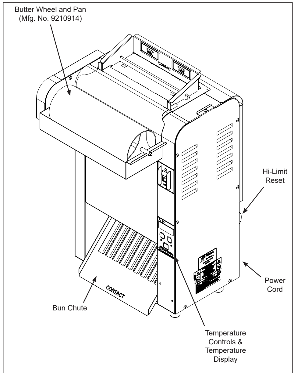
Figure 4. VCTM-2 Toaster
