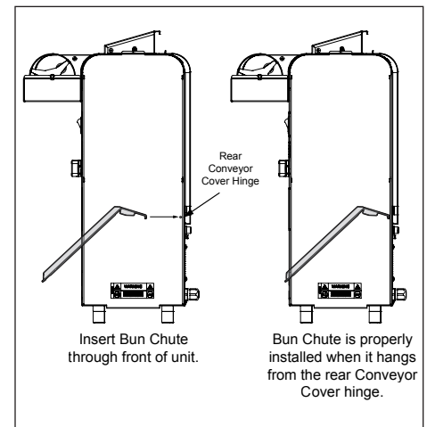
Figure 2. Installing Bun Chute
